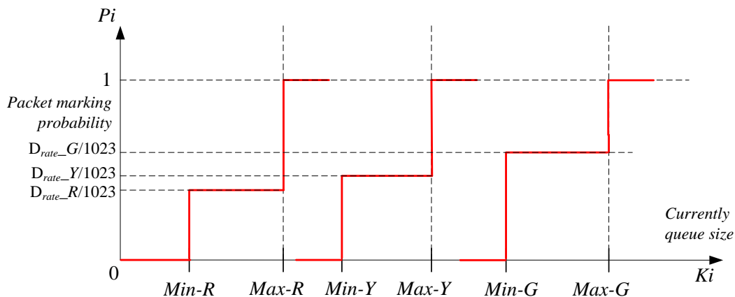
Figure 15. SWRED Packet Marking Probability of Different Drop Precedence
