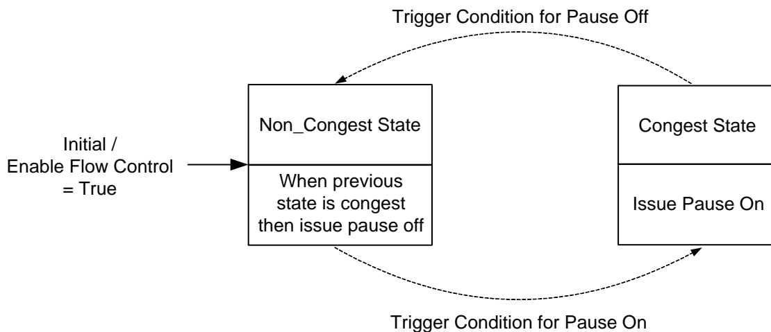
Figure 14. Flow Control State Machine
