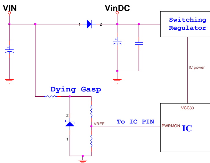
Figure 17. OAM Dying Gasp Application Circuit
