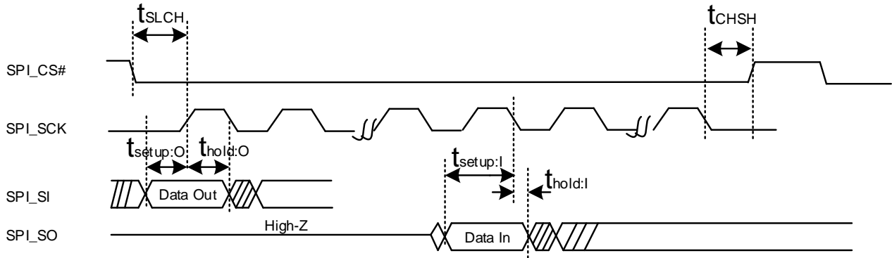
Figure 19. Master SPI Flash Controller Interface Timing
