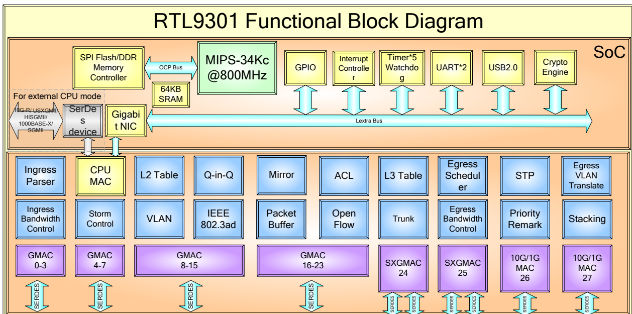
Figure 2. RTL9301 (48G+4*10G) Functional Block Diagram
