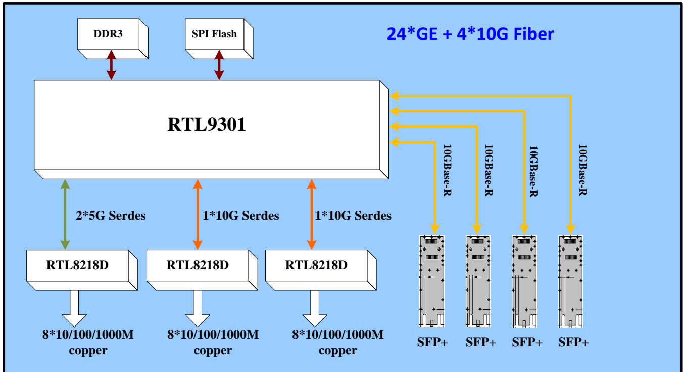
Figure 3. 24 10/100/1000Base-T + 4 10G Fiber
