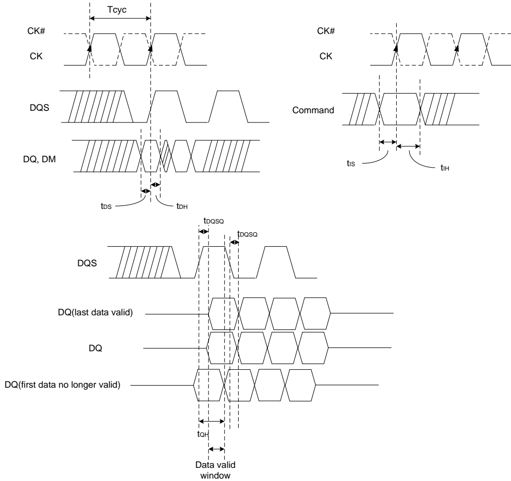
Figure 18. DDR3 Timing
