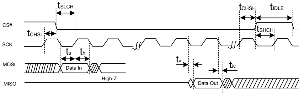
Figure 20. Slave SPI Flash Controller Interface Timing
