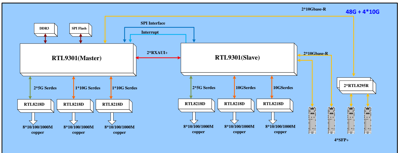
Figure 4. 48 10/100/1000Base-T + 4 10G Fiber
