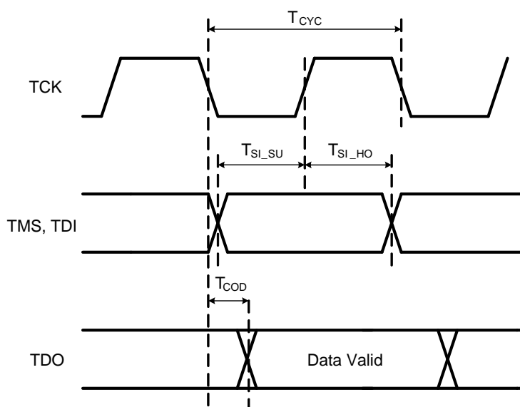
Figure 21. EJTAG Timing
