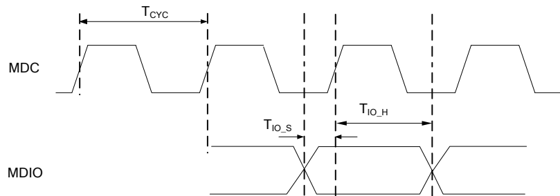
Figure 24. Scan LED timing
