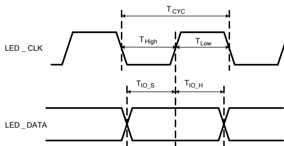
Figure 23. Serial LED Timing
