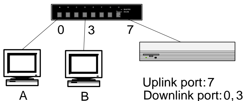
Figure 11. Port Isolation Example
