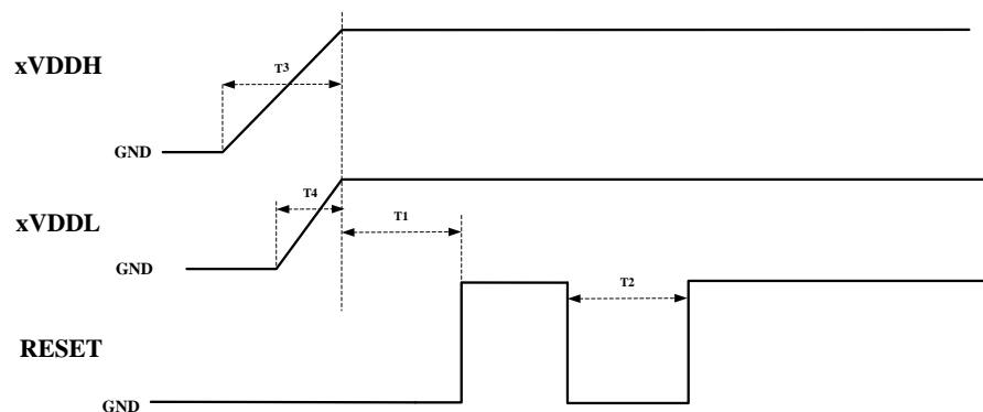
Figure 25. Power and Reset Timing
