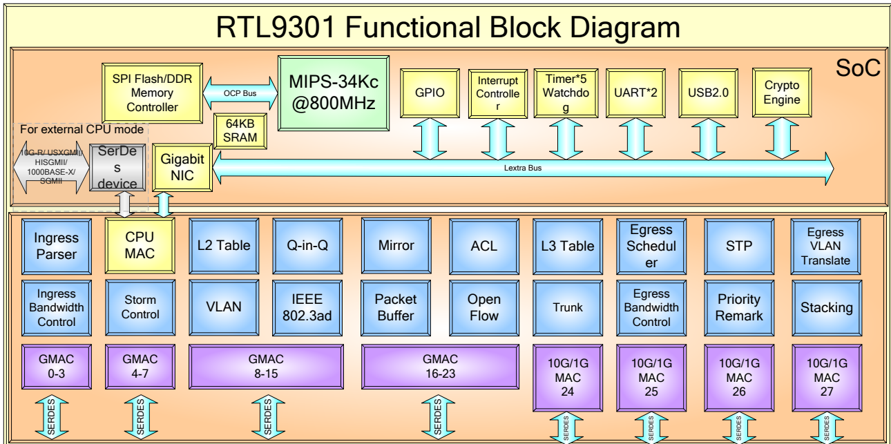
Figure 1. RTL9301 (24G+4*10G) Functional Block Diagram
