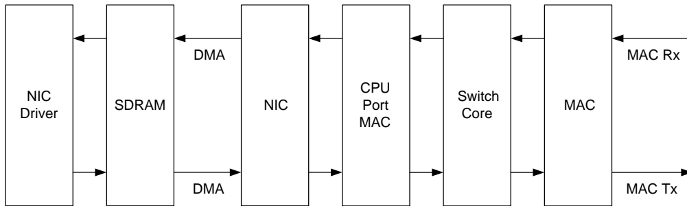
Figure 16. NIC Architecture
